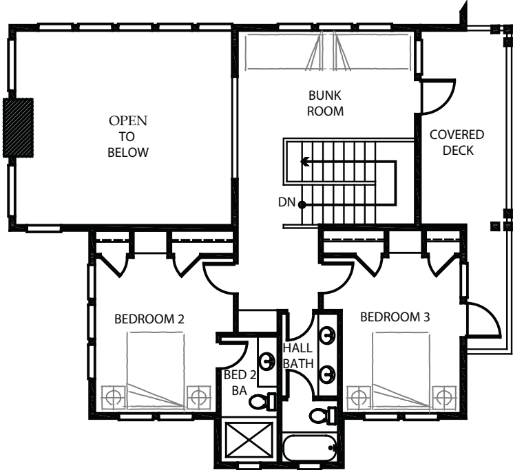
Upper Floor
